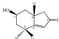
Loliolid (HP10)
