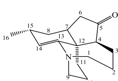
Fawcettidin (HP1)
